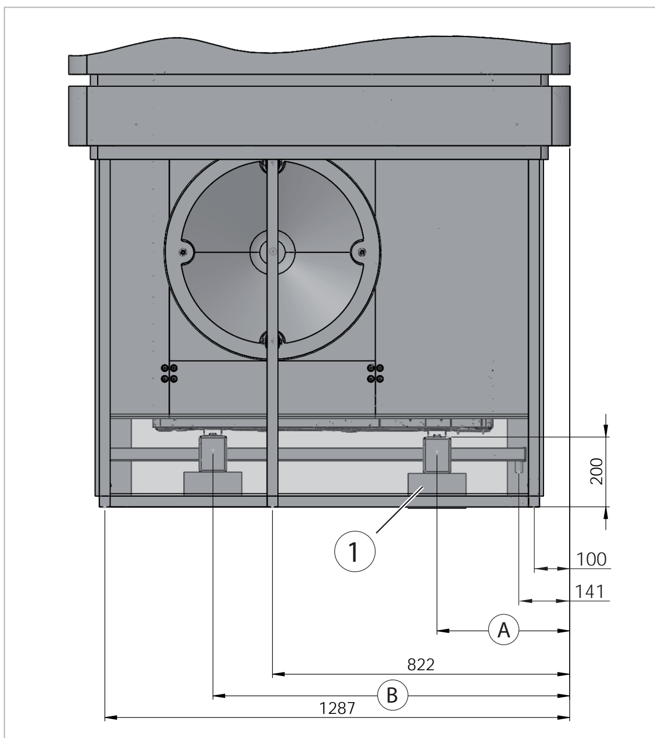
Fig. 3: Noise protection hood SWK 5.1 and SWK 7.1 front view (all dimensions in mm)
