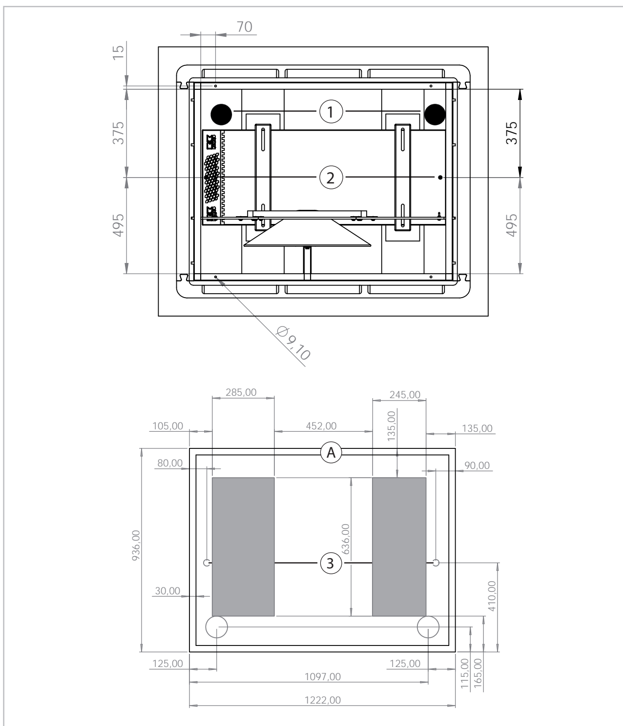
Fig. 10: Strip foundation SWK 5.1 and SWK 7.1
