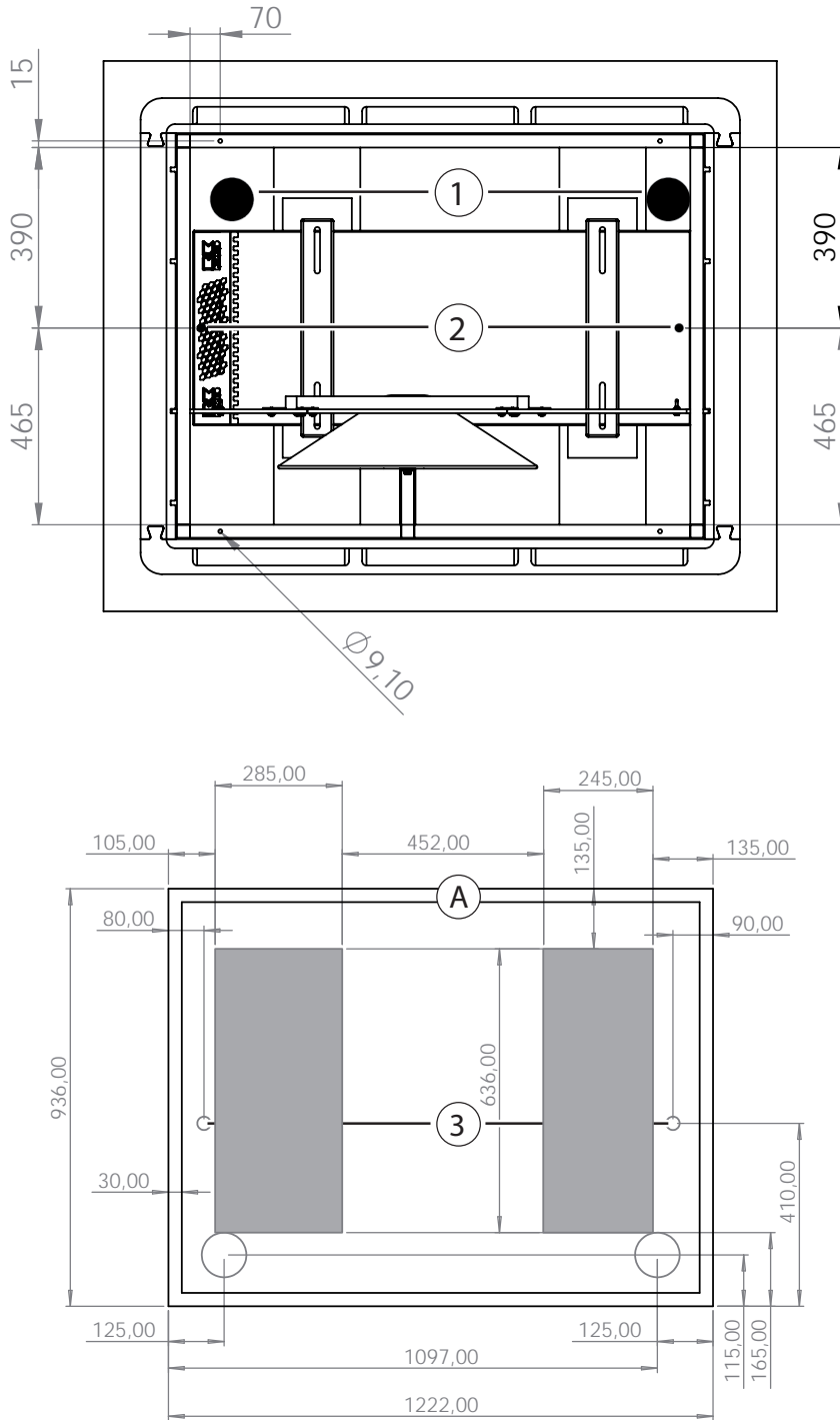
Fig. 9: Strip foundation SWK 4.1
