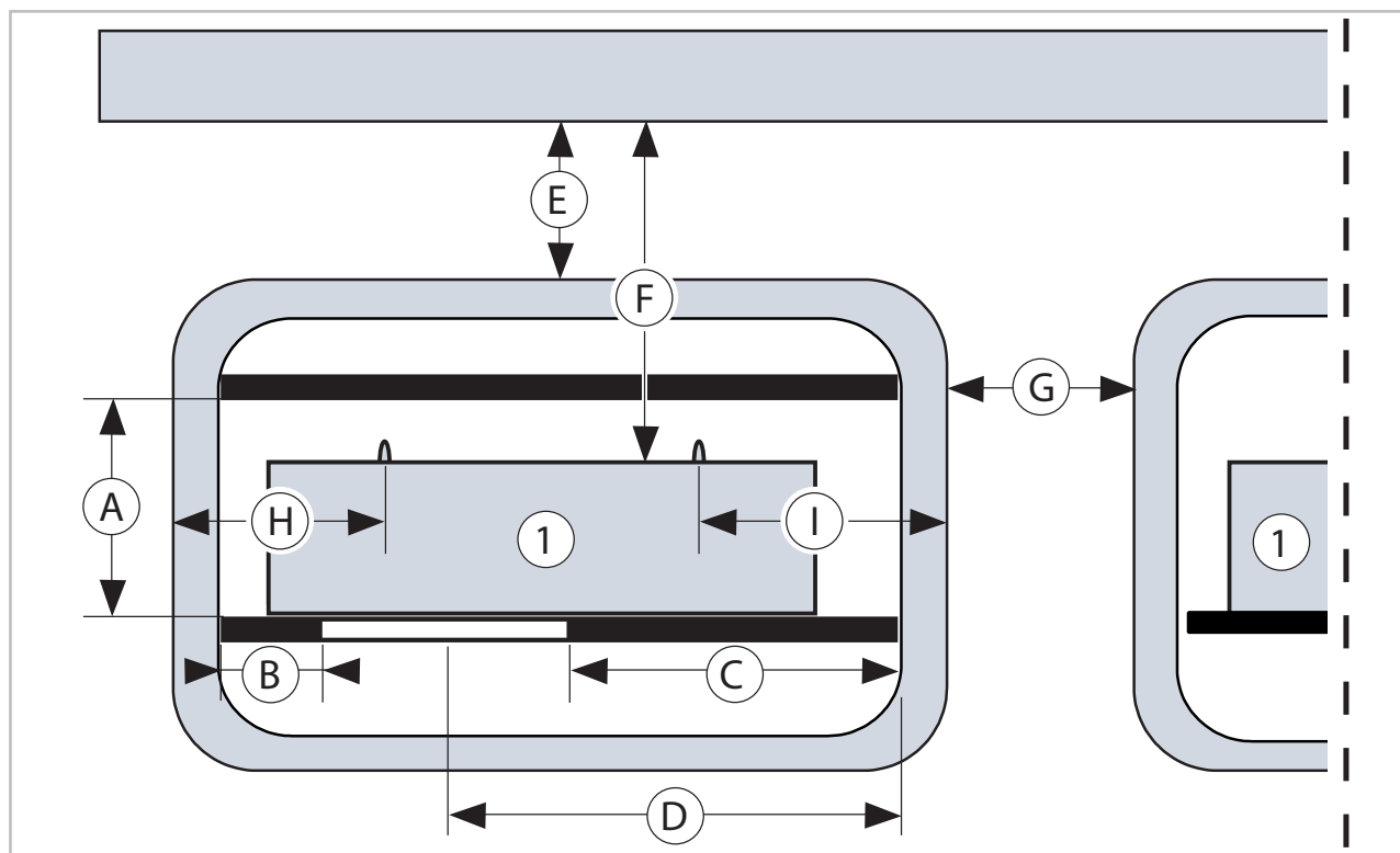
Fig. 4: Noise protection hood with outdoor units dimensions (all dimensions in mm)
