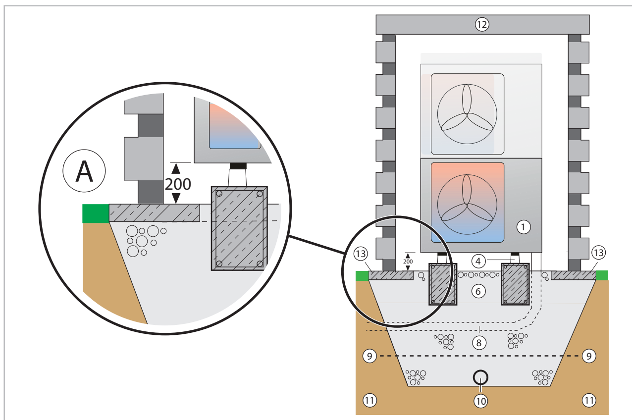
Fig. 8: Strip foundation (section)
