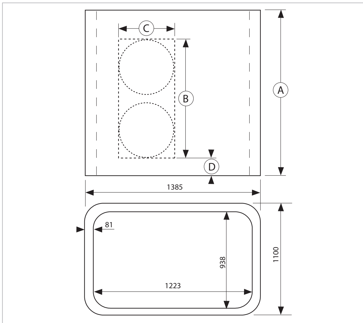
Fig. 1: Noise protection hood dimensions (all dimensions in mm)
